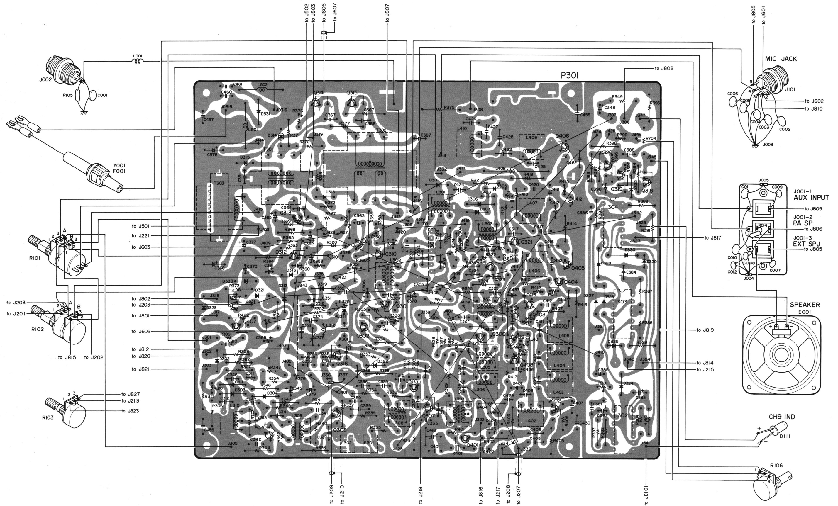
Figure 13 Circuit Board Diagram.
