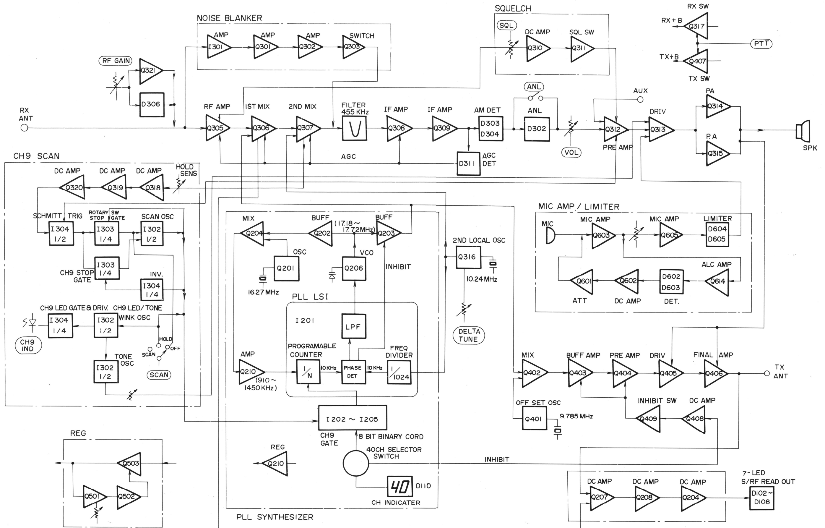
Figure 12 Overall Block Diagram.
