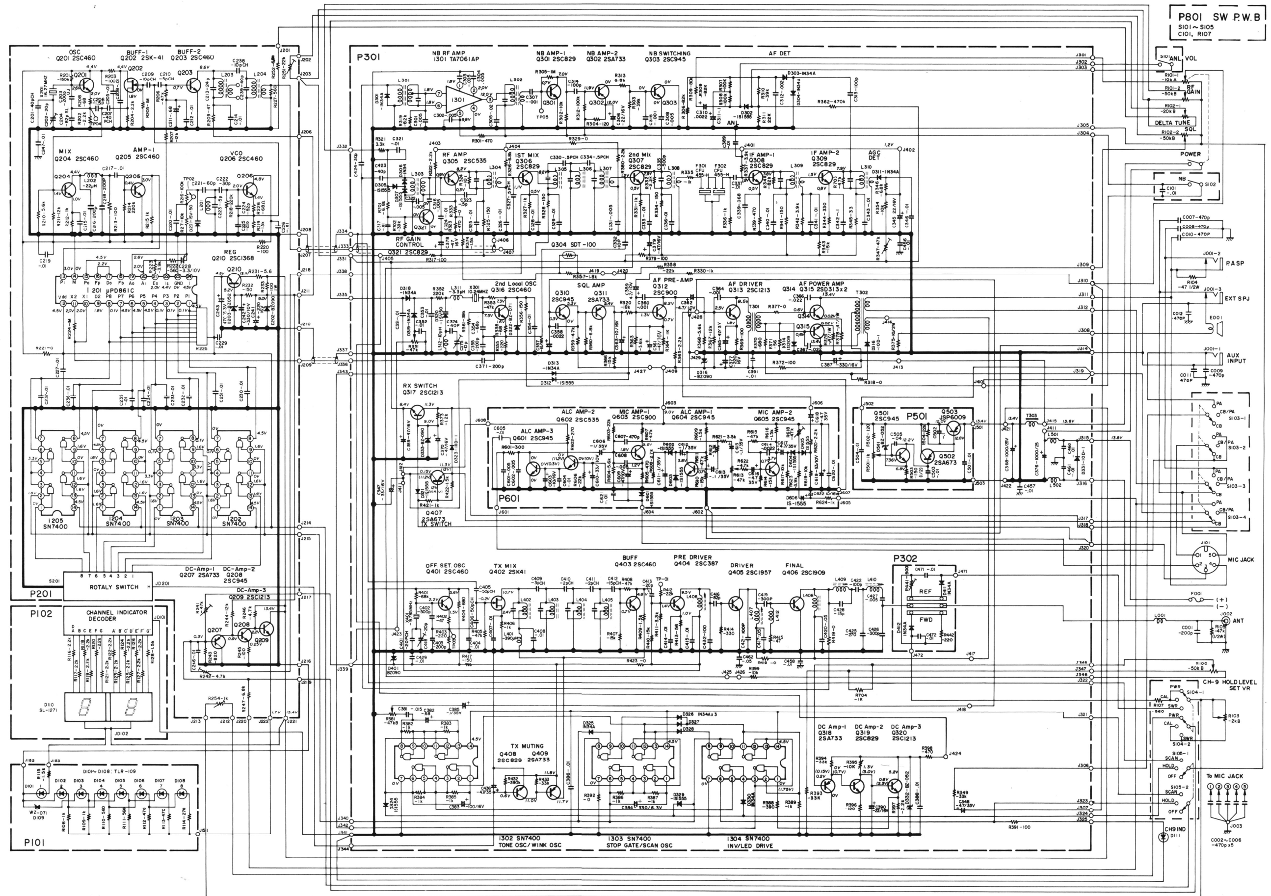
Figure 22 Schematic Diagram.
