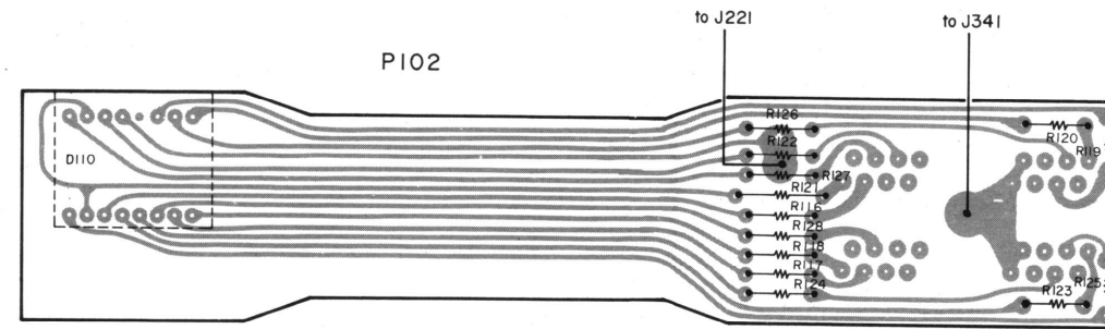
Figure 15 Seg Led Assembly-P102 Component Locations.
