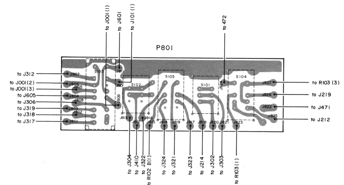
Figure 20 Switch Assembly-P801 Component Locations.
