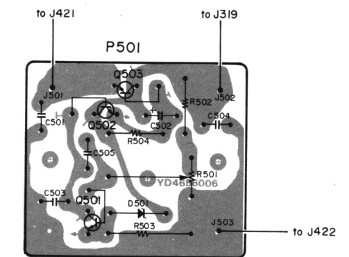
Figure 18 Regulator Assembly-P501 Component Locations.
