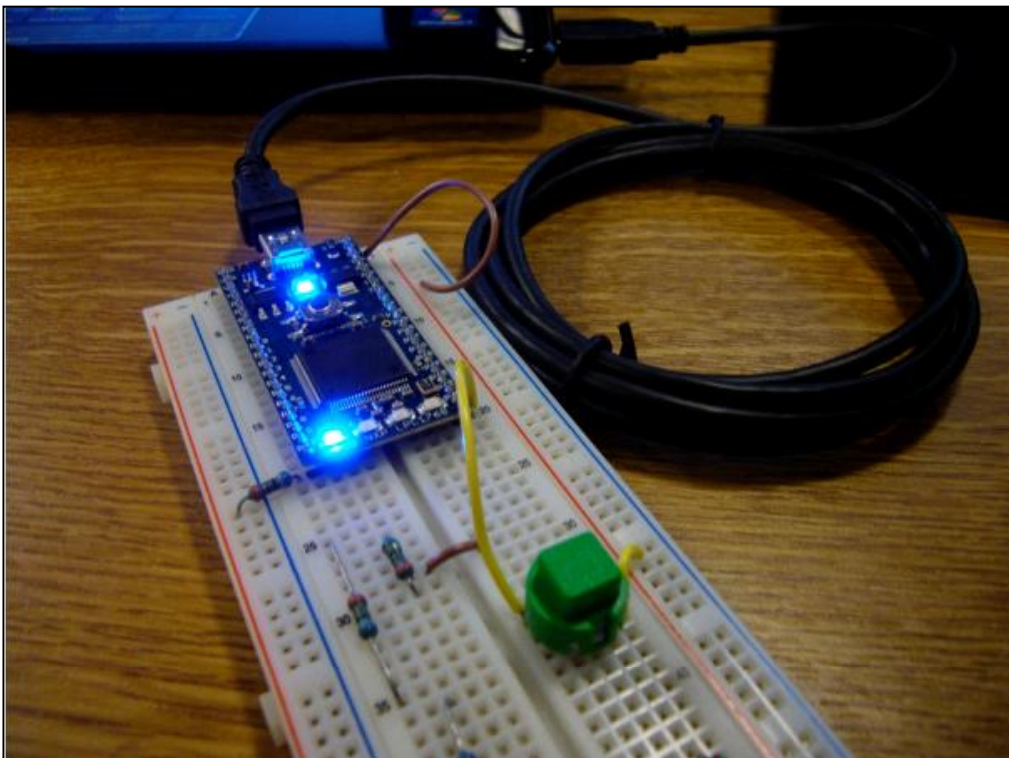
Figure 7: Photo du Mbed
