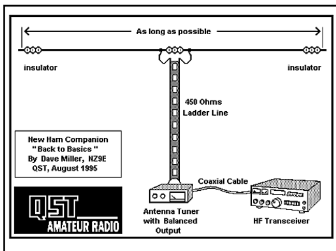
Figure 1 - Cut a long length of multi-stranded copper wire into two equal pieces. Attach the pieces to each end of a plastic or ceramic insulator and place two more insulators at the two ends. Attach 450 Ohms ladder line at the center and run it back to your antenna tuner. Secure ropes to both ends and raise the antenna as high as you can. You now have a dipole antenna that you can use on several HF bands.
