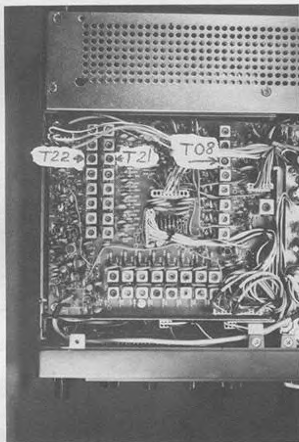
RF board
